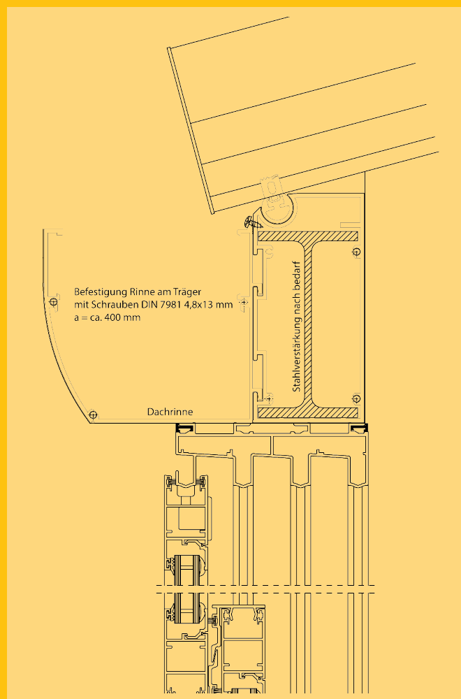
Roof gutter and beam with sliding doors
