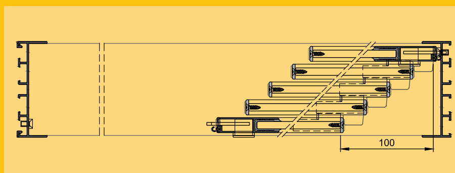
Frameless all-glass sliding system, opened
