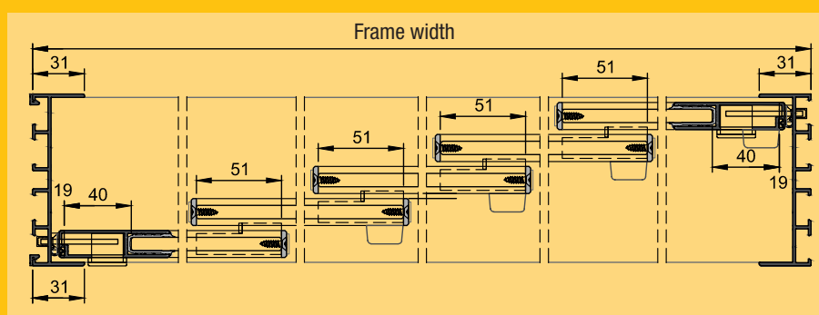
Frameless all-glass sliding system, closed
